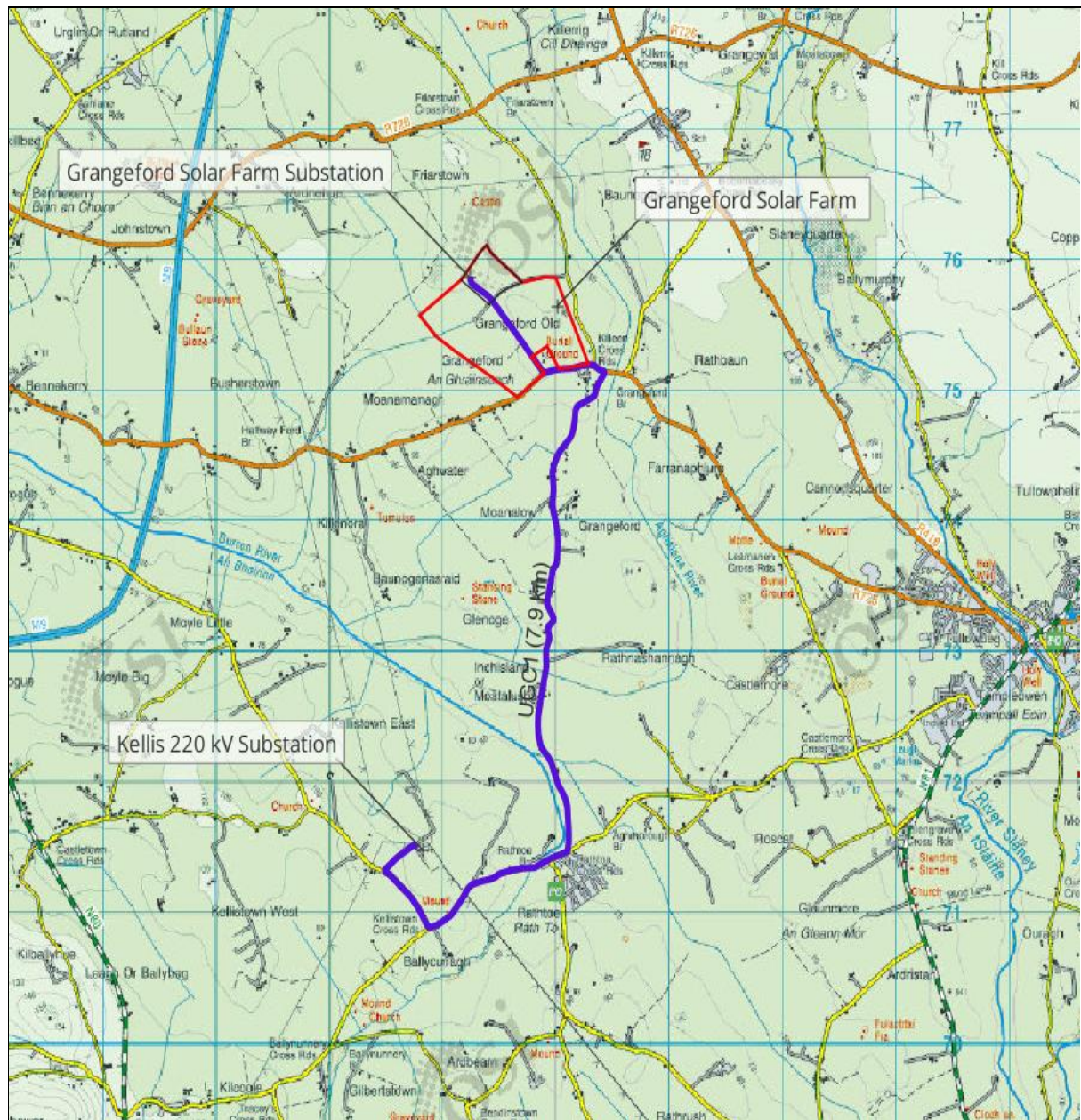
Figure 1 - Proposed Grid Connection Route
