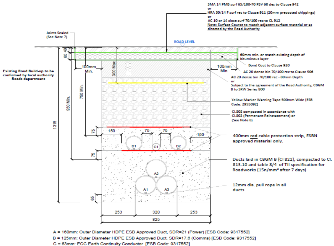
Figure 3 - Typical Trench in Road Section
