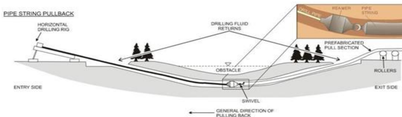
Figure 14 - Typical HDD Installation (not to scale)
